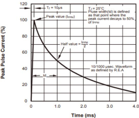
Fig.3 - Pulse Waveform
